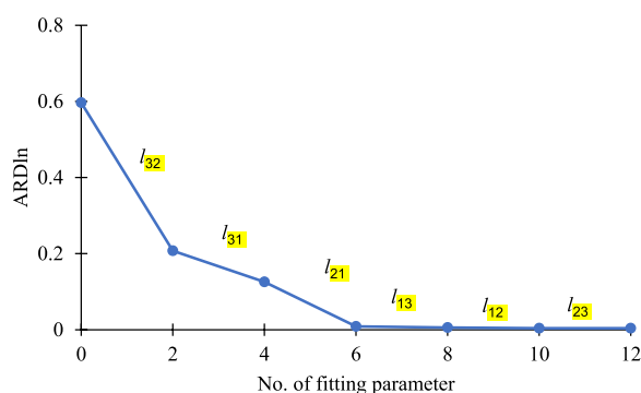
Fig. 6 Xanthone–tricaprin–tricaprylin interaction analysis via the local composition–regular solution theory (LC-RST) model
