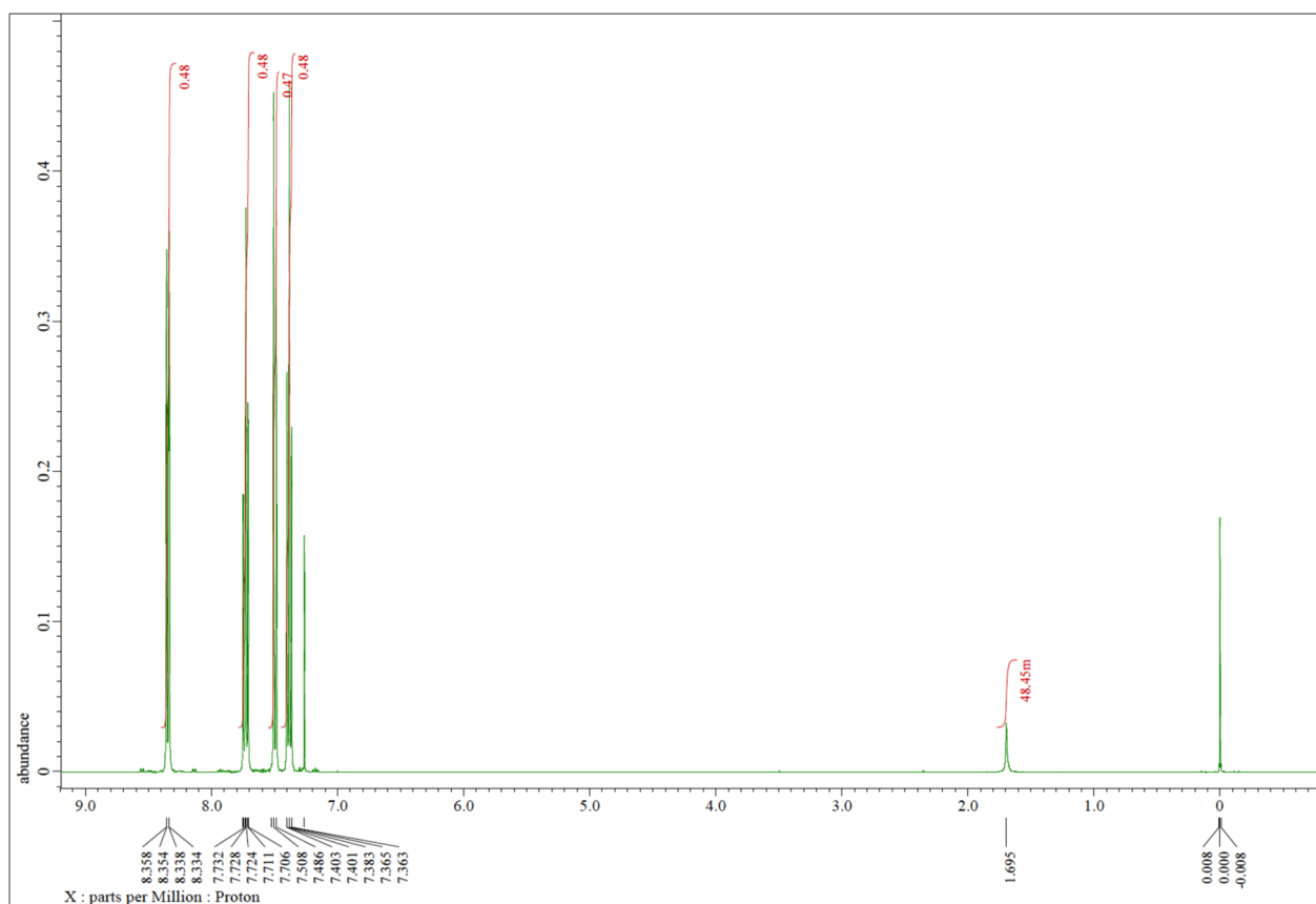
Fig. 8 Nuclear magnetic resonance spectrum of standard xanthone
