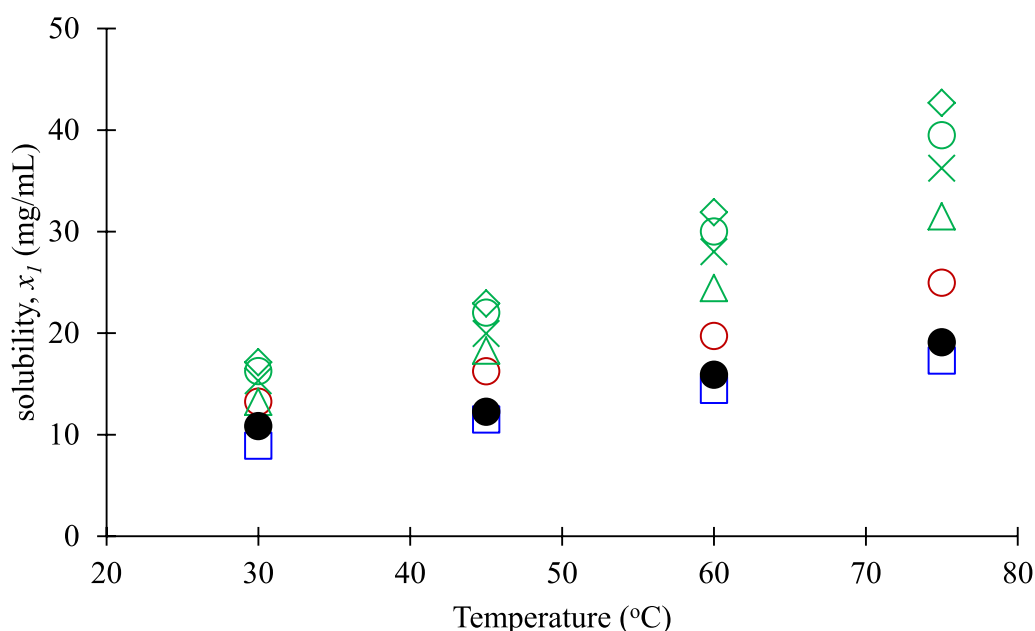
Fig. 4 Solubility of xanthone (1) in a mixture of tricaprin ( x_2 ): tricaprylin ( x_3 ) as a function of temperature. □ (1:0); △ (0.77:0.23); ◇ (0.55:0.45); ○ (0.36:0.64); × (0.17:0.83); ○ (0:1); ● (virgin coconut oil)
