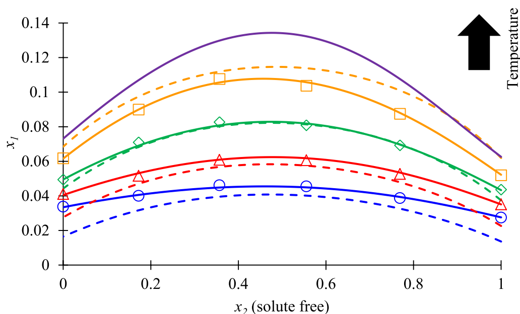
Fig. 5 Solubility profile of xanthone ( x_1 ) in a mixture of tricaprln ( x_2 ); tricaprylin ( x_3 ). Markers: experiment; smoothed line: local composition regular theory model (LC-RST) with significant fitting parameters ( l_{23} was removed); dashed line: Wilson model. ■ : 75 °C (orange); ◆ : 60 °C (green); △ : 45 °C (red); ○ : 30 °C (blue). x_2 (solute free) is the mole fraction of tricaprln (2) in the mixed solvent that is free of xanthone. (Raw data: Table S3). Purple: 90 °C (predicted with LC-RST)
